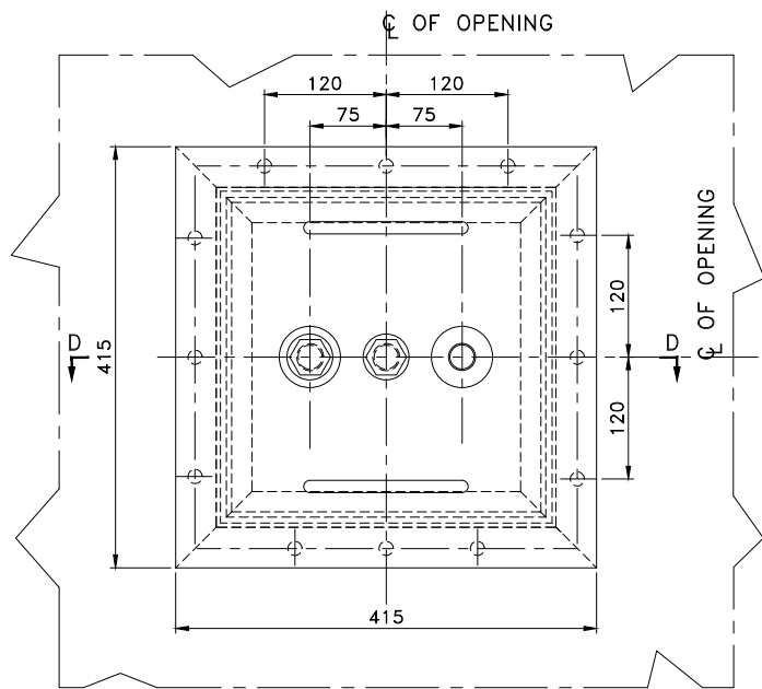
FLUIDISING PAD FIXING ARRGT. FOR 300 X 300 OPENING (TOTAL QTY.2 NOS/HOPPER)
