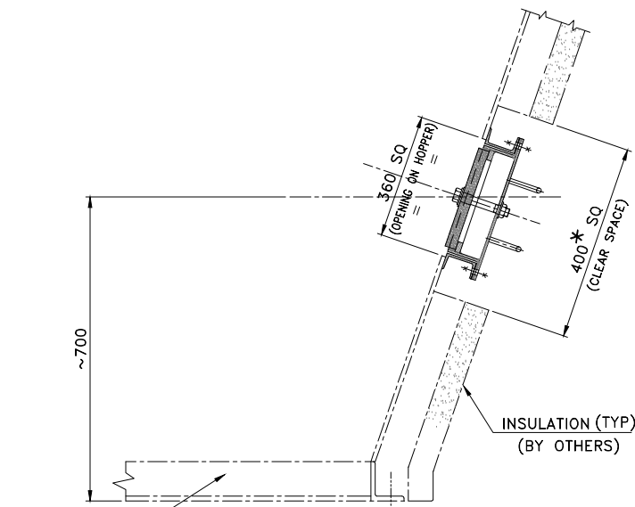
SECTION Z-Z
