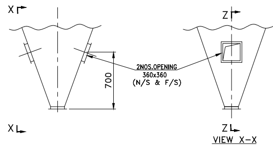
SCHEMATIC LAY OUT OF FLUIDISING PADS WITH OPENINGS ON ESP HOPPER WALLS (AS PER BHEL DRG. NO.0-00-111-27437)
