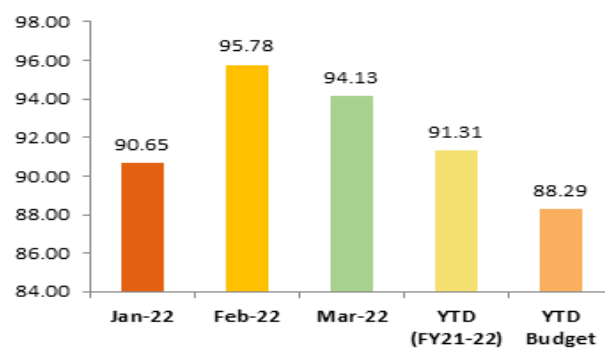
Plant Availability Factor (%)
