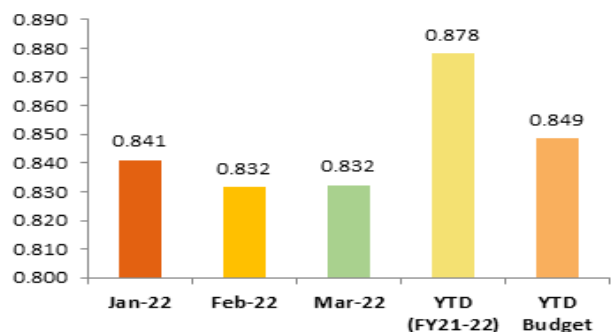
Sp. Coal Cons. (kg/kwh)
